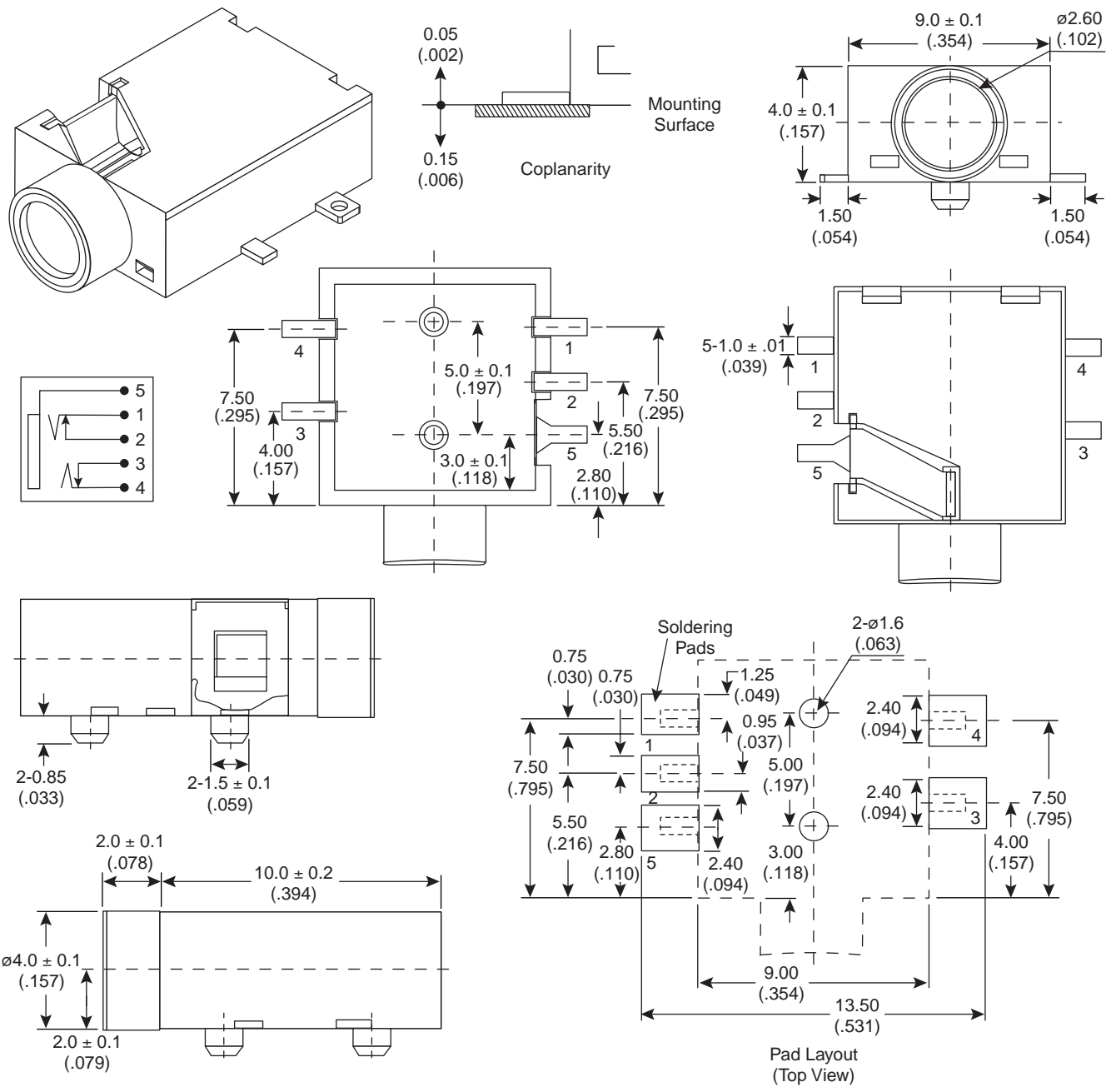
Dimensions mm and (In.)
